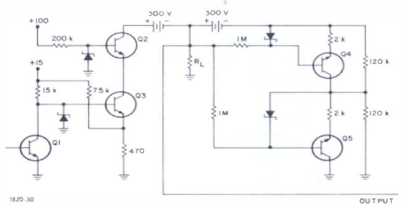
Figure 6. Simplified schematic diagram of the output amplifier.
