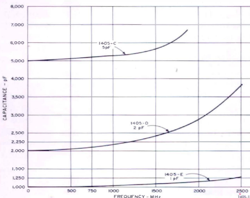
Figure 3. Capacitance-vs-frequency characteristics of 1405 capacitors.
