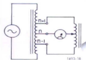
Figure 7. Principle of "straddling" method.
