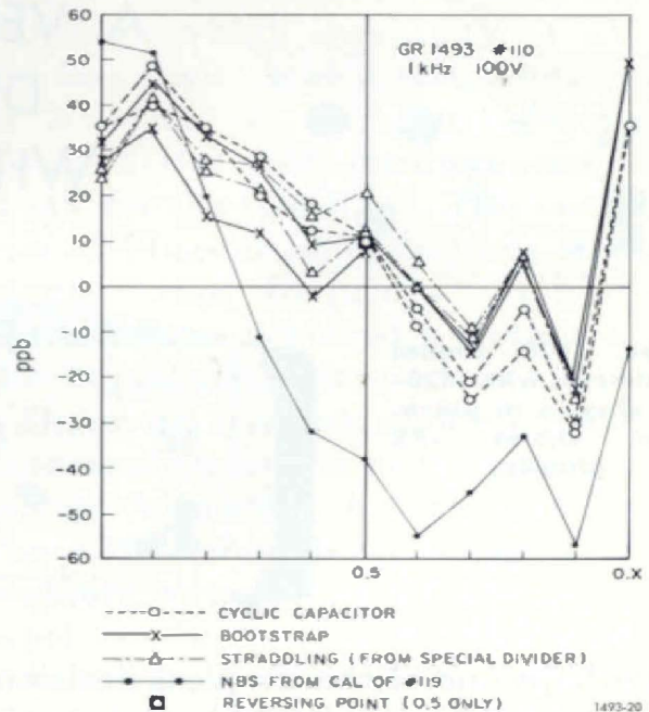
Figure 9. Results of six calibrations, two using each method. Correction in parts-per-billion plotted vs ratio.
