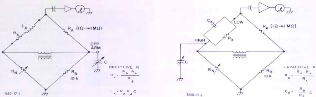
Figure 1. Diagrams showing use of the ac-resistance bridge to make reactive balances.
