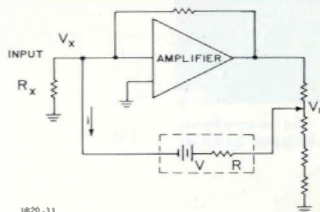
1820-31 Figure 7. Resistance-measurement technique with the 1820-P1.
