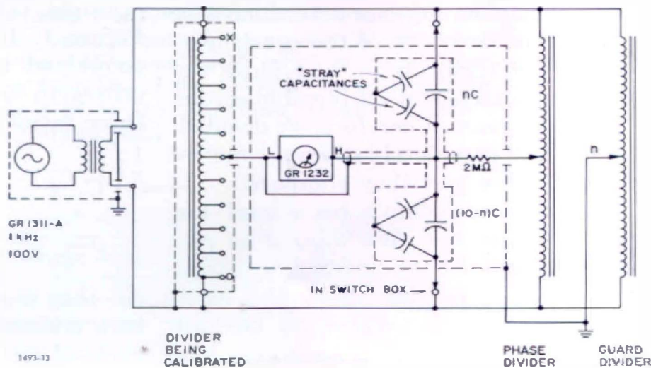
Figure 2. Connection diagram for "cyclic capacitor" method (note: n = number of tenths of input).
