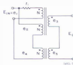
Figure 4. Simplified diagram of "two-stage" transformer, which is actually two transformers interconnected.
