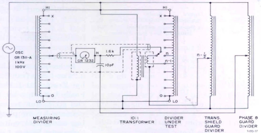
Figure 6. Connection diagram for "bootstrap" method. (Note: n = number of tenths of input. At midpoint n = 5 and n - \frac{1}{2} = 4.5 , which is a ratio of 0.45).
