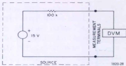
Figure 2. Input impedance of DVM is critical in measurement such as that indicated here (see text).
