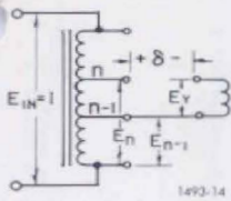
Figure 3. Basic principle of "bootstrap" method, where E_y is the voltage obtained from the shielded 10:1 transformer.
