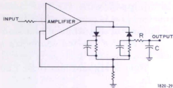
Figure 8. Basic circuit diagram of the operational rectifier of the 1820-P2.
