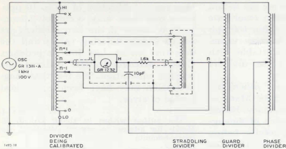
Figure 8. Connection diagram of "straddling" method.
