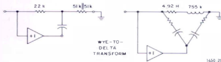
Figure 3a (left). Bridge can be used to determine input impedance of transistor amplifiers such as the bootstrapped emitter follower shown here. Figure 3b (right). A redrawing of the circuit of Figure 3a, showing why the input appears inductive.
