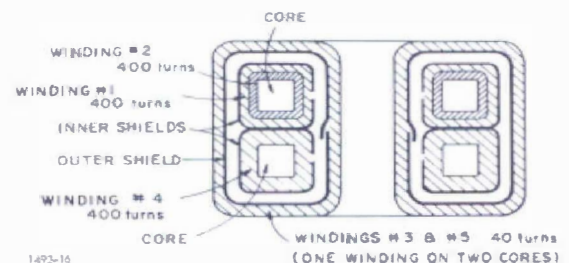
Figure 5. Cross-section diagram of "two-stage" transformer. Note two toroidal cores used.
