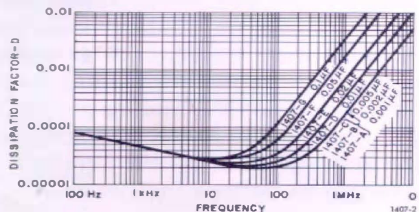
Figure 2. Dissipation-factor-vs-frequency characteristics of the 1407 capacitors.
