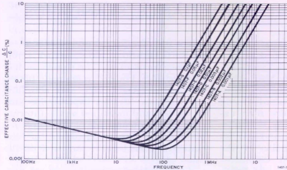
Figure 1. Capacitance-vs-frequency characteristics of the 1407 capacitors.
