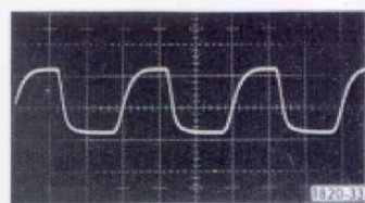
Figure 5. Ac waveform at photochopper output.
