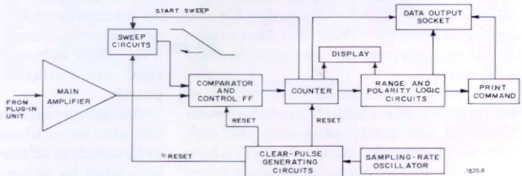
Figure 3. Simplified block diagram of the 1820.
