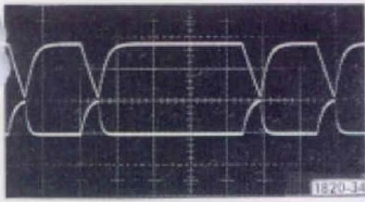
Figure 4. Oscilloscope showing the linear (top) and log (bottom) sweeps of the 1820.
