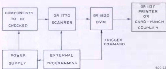
Figure 10. Typical system for measuring capacitor leakage current.
