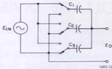
Figure 1. Simplified diagram of capacitive divider using only three capacitors.
