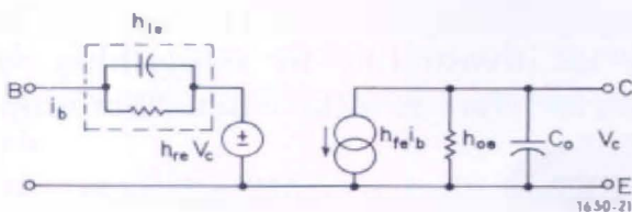
Figure 4. h-parameter equivalent circuit of a transistor.
